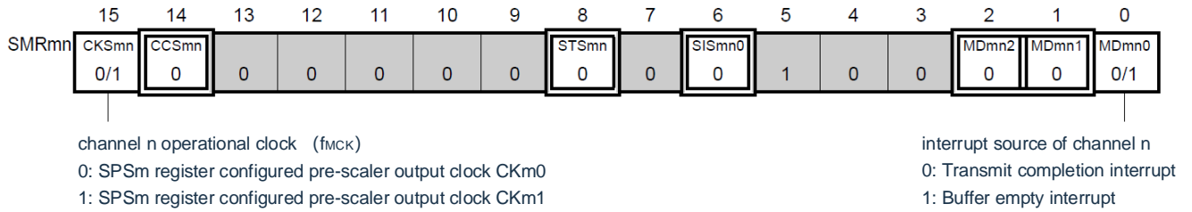
Figure 19-25 3-wire Serial I/O (SSPI00, SSPI01, SSPI10, SSPI11, SSPI20,SSPI21) Example of register setting content when master sending
