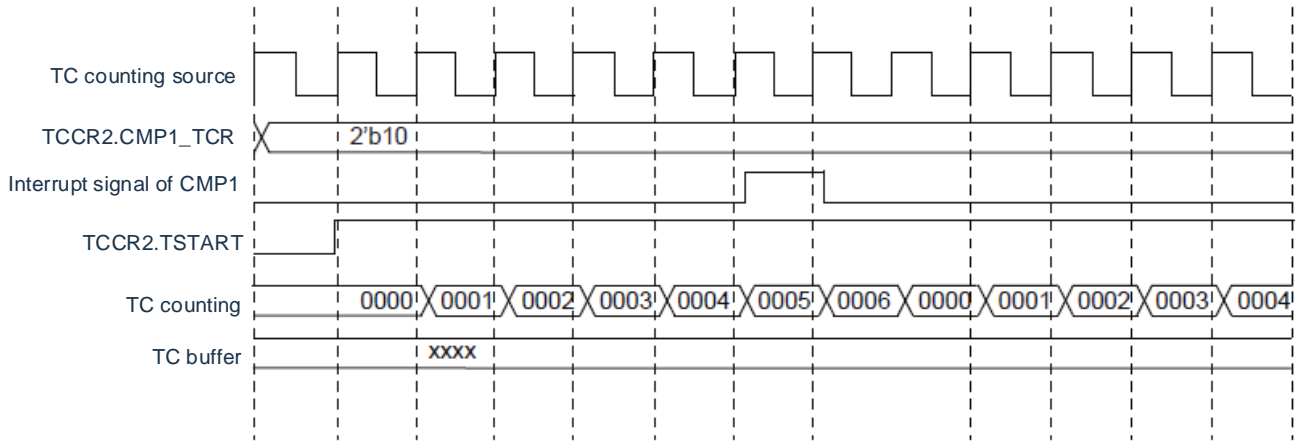
Figure 9-16 Example of CMP1 triggering a Timer C count reset
