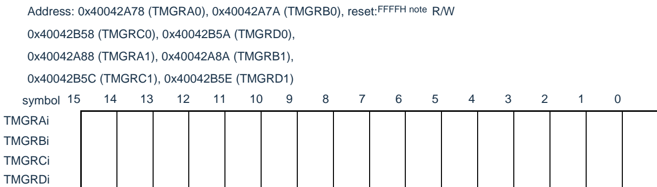
Figure 10-34 timer m general register ai, bi, ci, di (TMGRAi, TMGRBi, TMGRCi, TMGRDi) (i=0,1) in [Input capture] format
