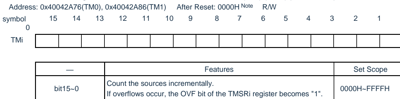
Figure 10-30 Format of timer M counter i(TM i ) (i=0,1) [timer mode]
