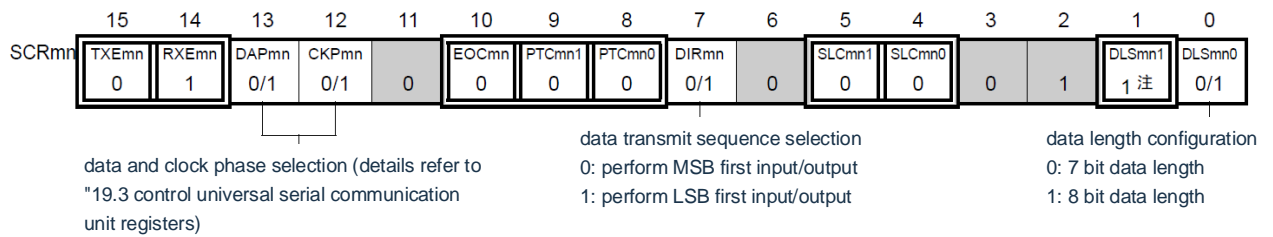
(b) serial communication operation configuration registermn mn(SCRmn)
