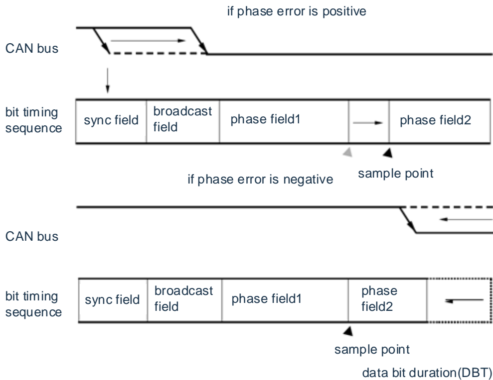
Figure 21-21. Resynchronization
