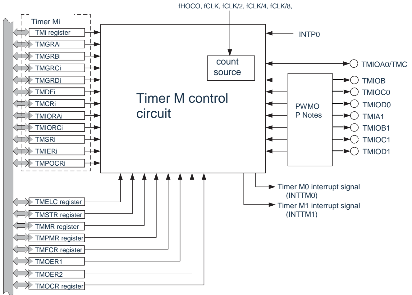
Figure 10-1 Block diagram of timer M
