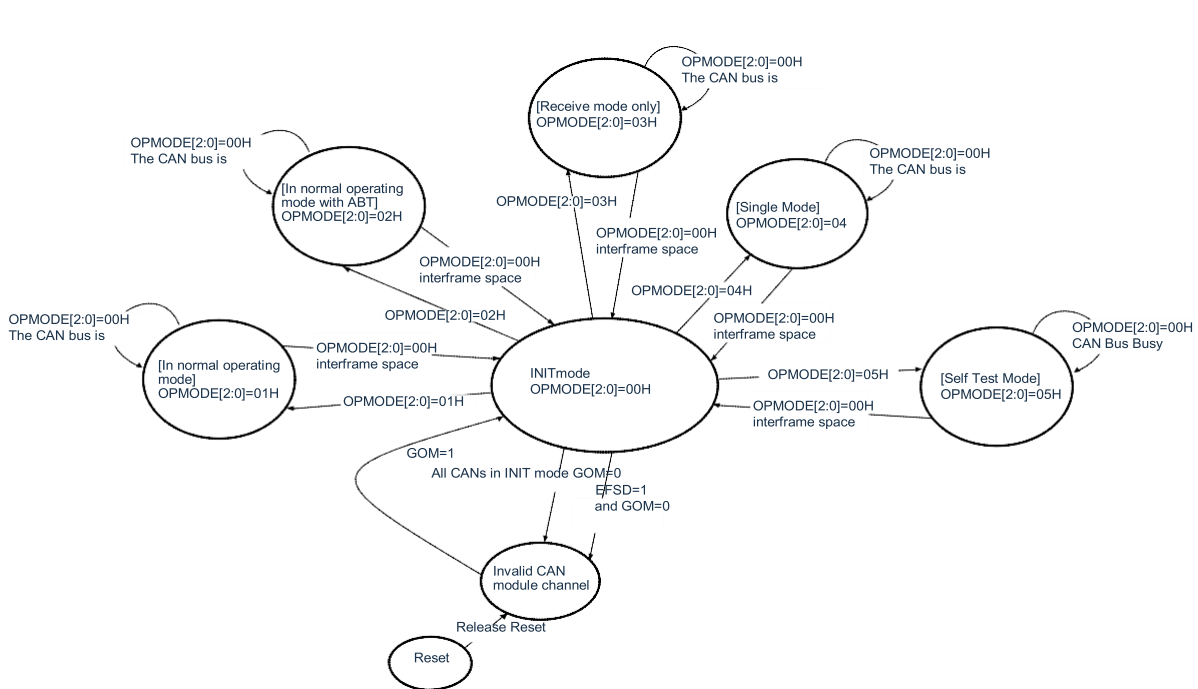
Figure 21-54. Transition to Operation mode
