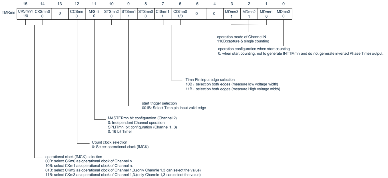
Figure 6-55 Example of register setting content when measuring high and low level width of input signal
