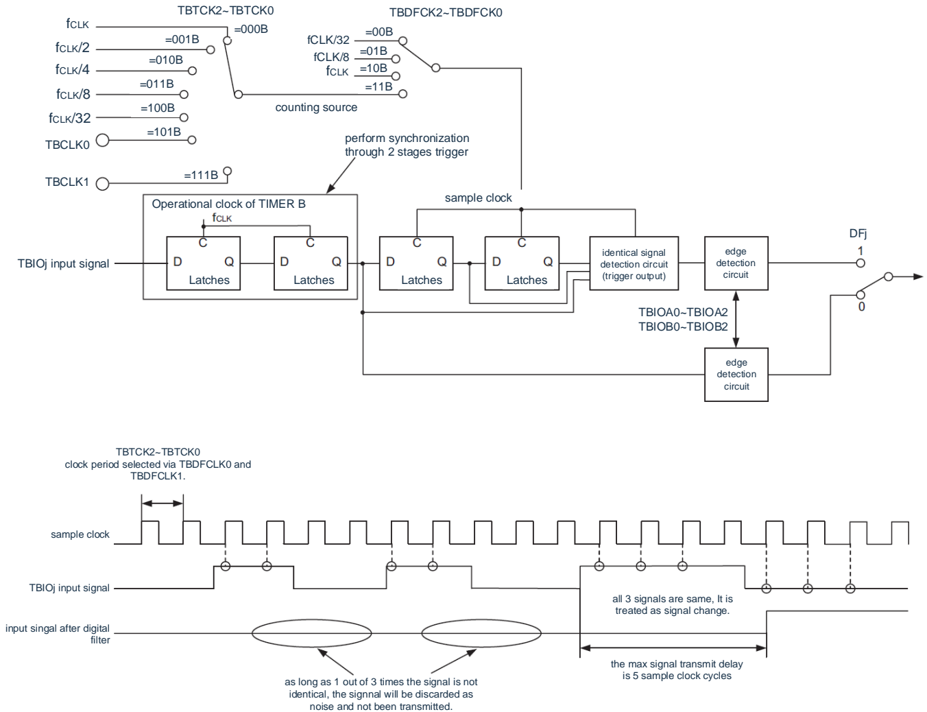
Figure 8-15 Block diagram of digital filter
