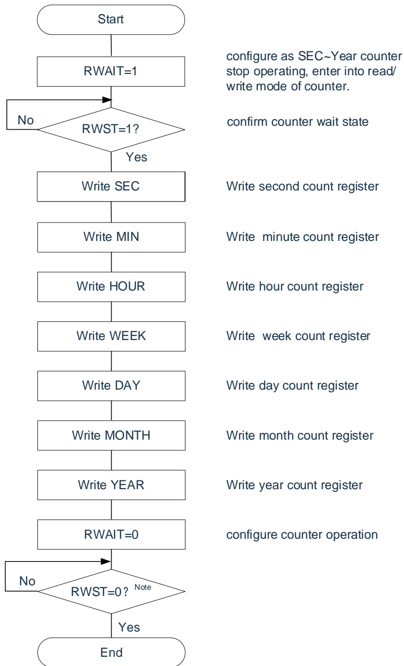
Figure 11-20 Read operation steps of real-time clock counter
