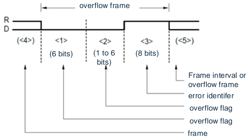
Figure 21-16. Overload frame
