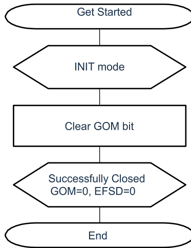
Figure 21-84. Normal shutdown handling
