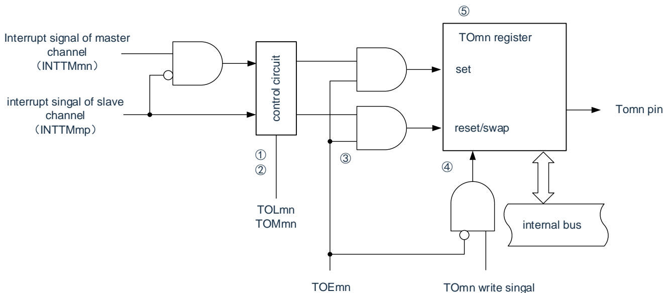
Figure 6-31 Structure of output circuit
