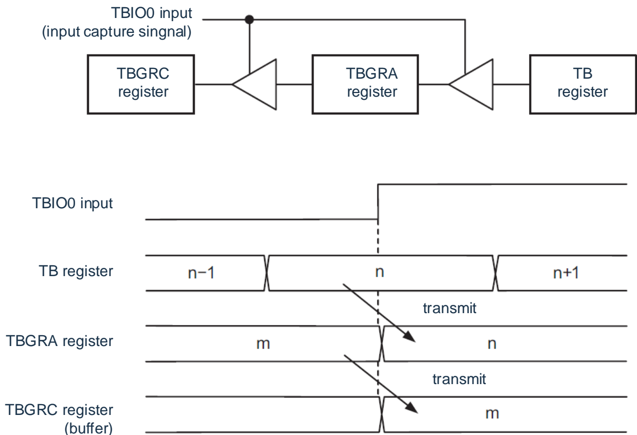
Figure 8-13 Buffer Operation for Input Capture
