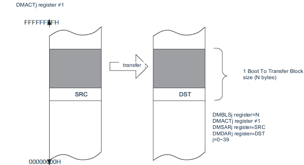
Figure 23-18 Repeat mode data transfer
