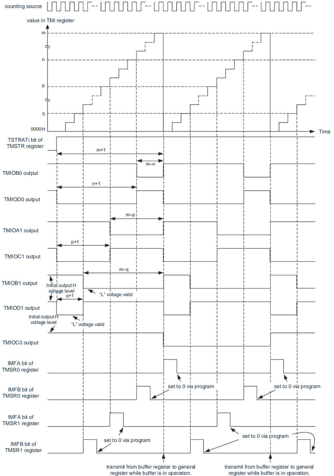
Figure 10-57 Operating example of reset synchronous PWM mode
