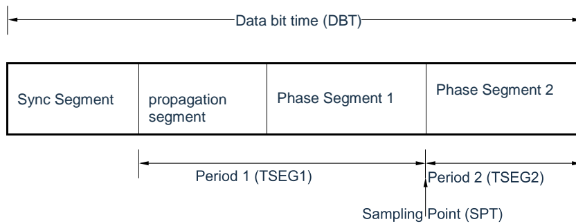
Figure 21-40. Data bit time
