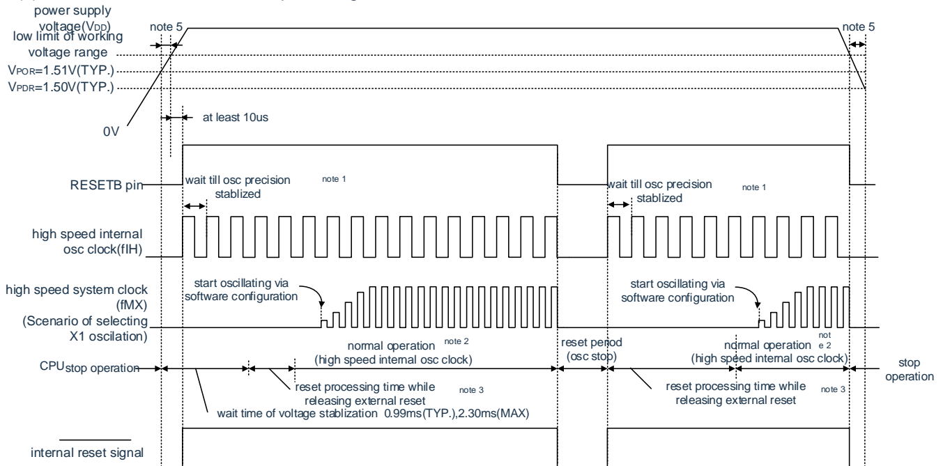
Figure 29-2 Generation sequence of internal reset signal of power-on reset circuit and voltage detection circuit (1/3)
