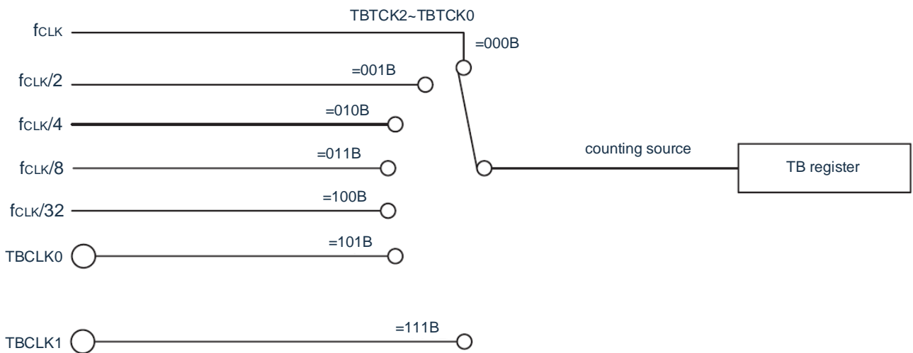
Figure 8-12 Block diagram of count source
