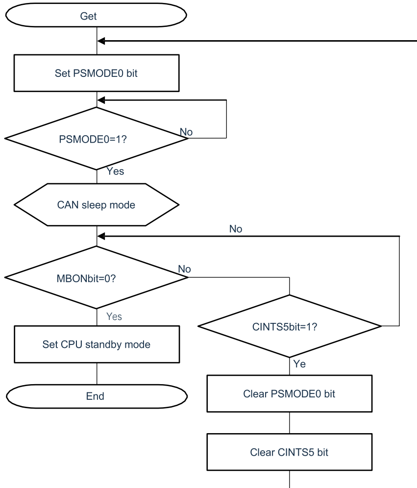
Figure 21-87. Setting CPU Standby (from CAN sleep mode)
