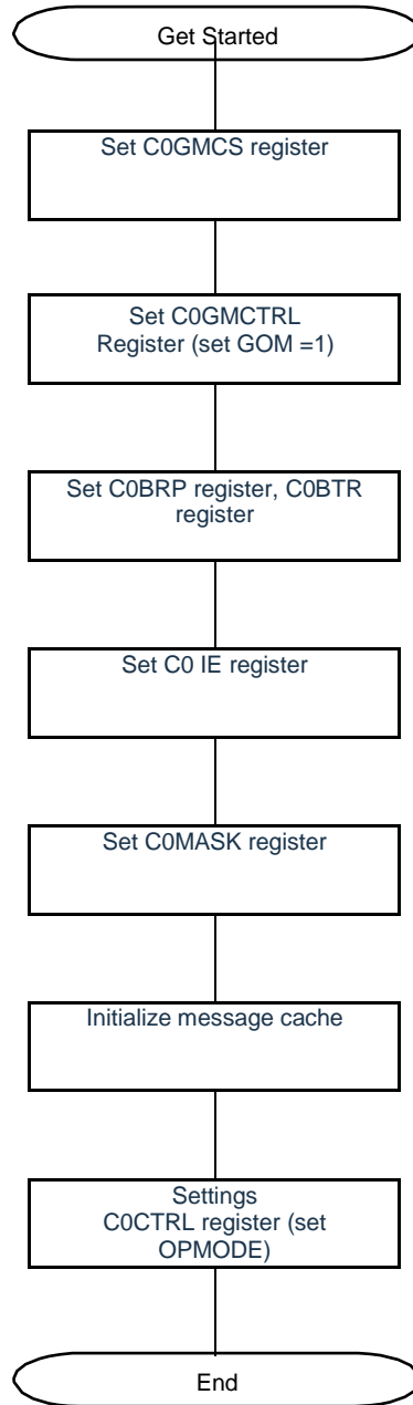
Figure 21-63. Initialization
