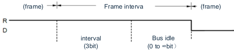
Figure 21-13. Interframe Space (Error Active Node)
