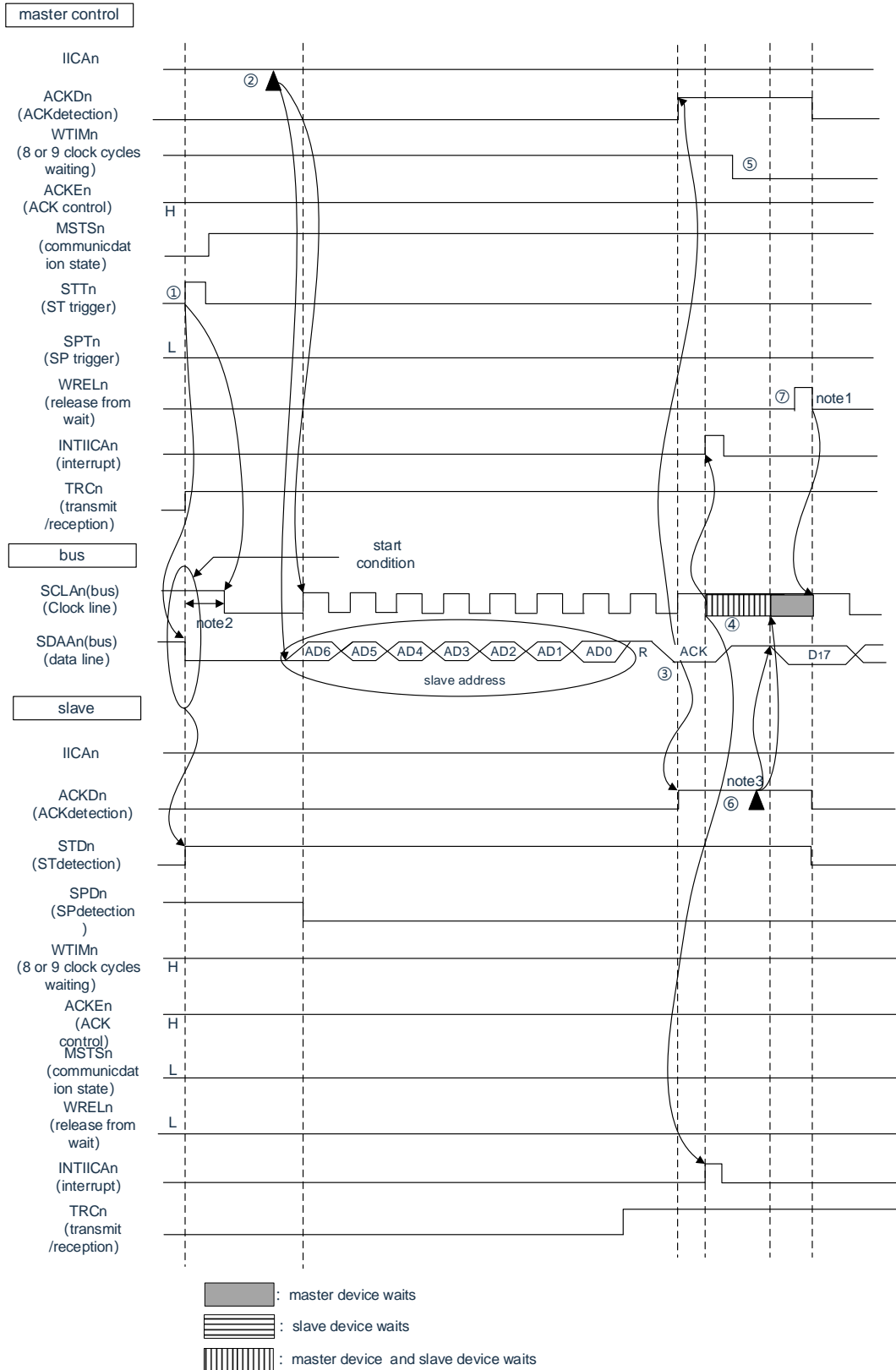
Figure 20-33 Example of communication for a slave master device (Main control equipment: Select 8-clock wait, slave: Select 9 clock wait) (1/3)
