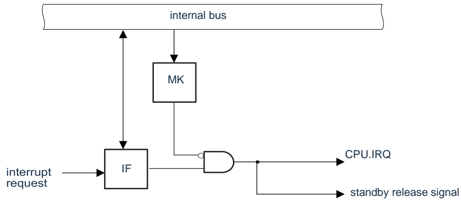
Figure 25-1 Basic structure of interrupt functionality
