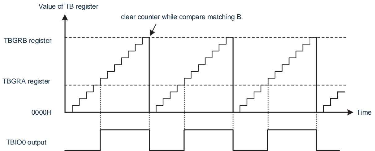
(b)clear counter while TBGRB register compare matching
