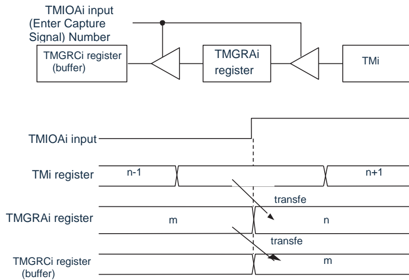
Figure 10-42 Buffer Operation for Input Capture
