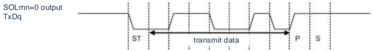
Figure 19-18 Example of Level Inversion for Transmitting Data
