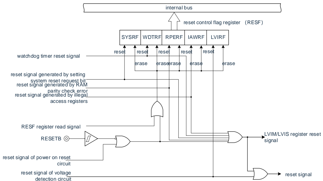
Figure 28-1 Block diagram for reset function
