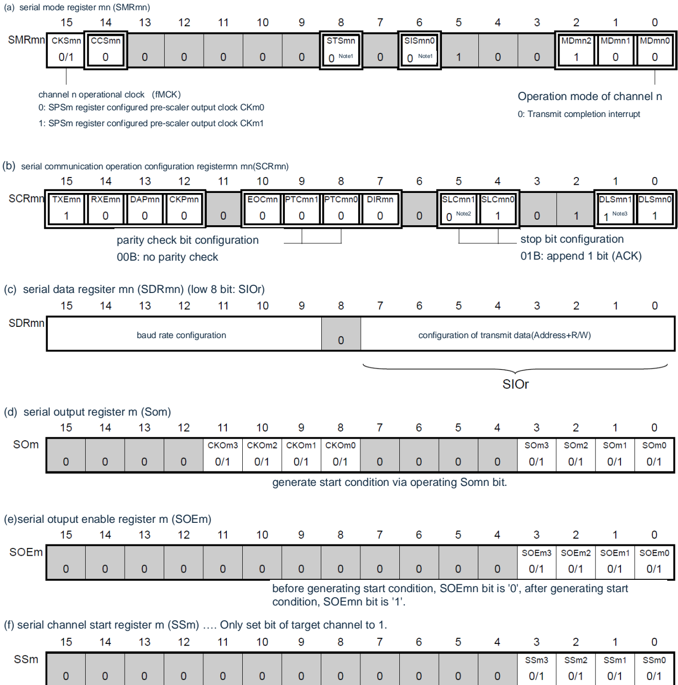
Figure 19-128 Simple I2C (IIC00, IIC01, IIC10, IIC11, IIC20, IIC21) address segments sent Examples of register setting content for
