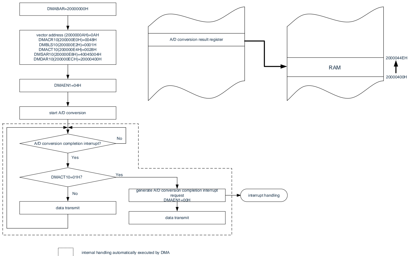
Figure 23-16 Example of normal mode use 1: Continuously taking A/D conversion results
