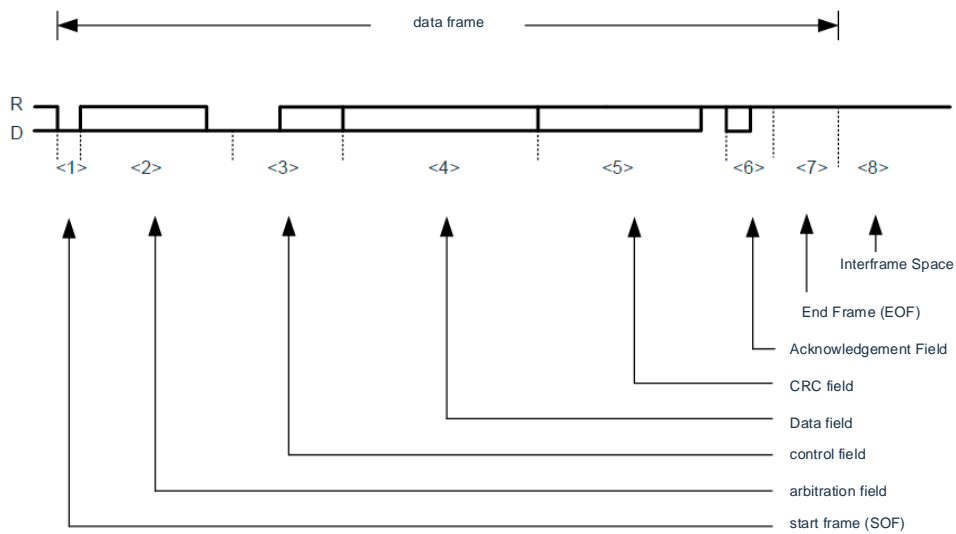
Figure 21-3. Data frame
