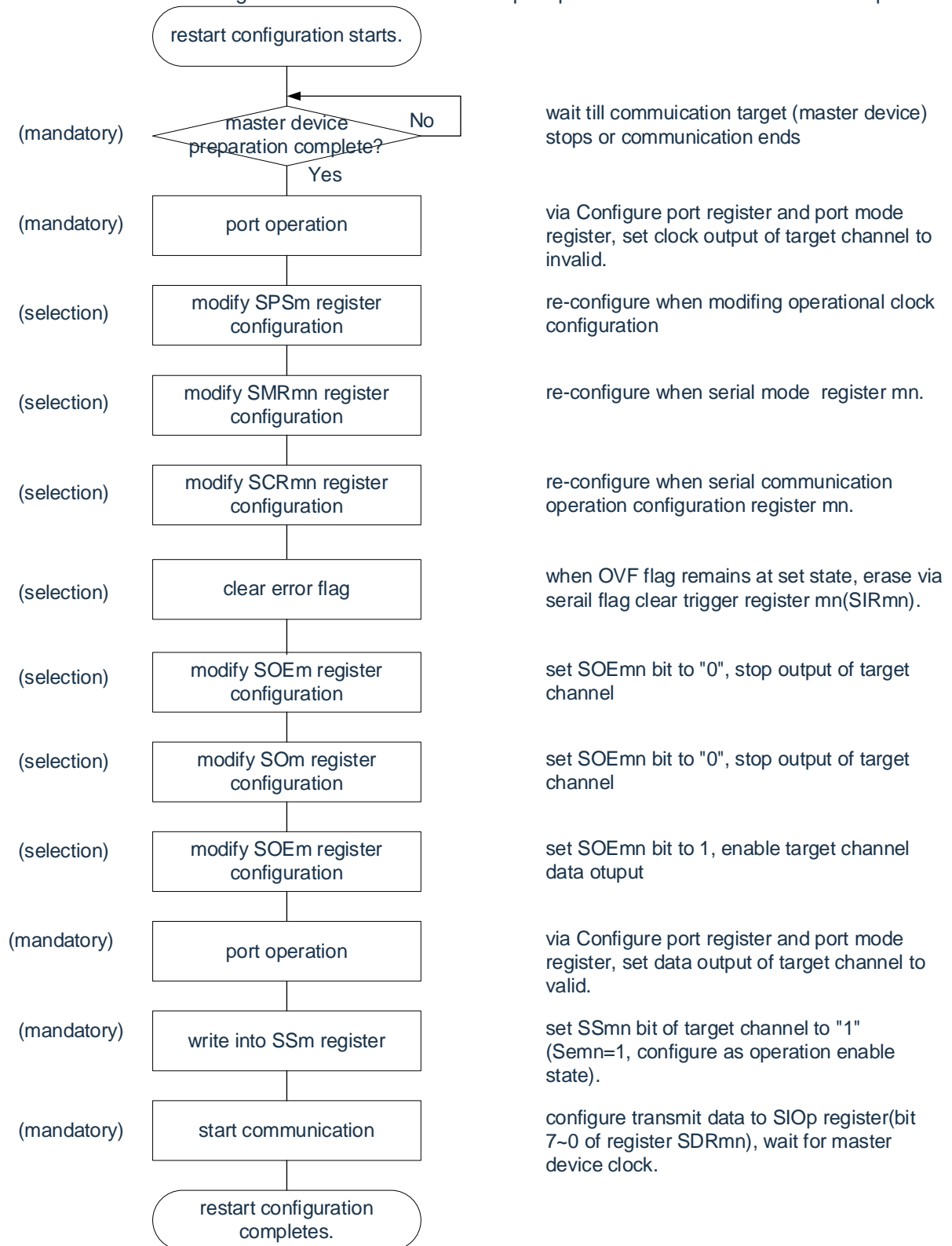
Figure 19-66 Restart the set-up steps for slave transmission and reception
