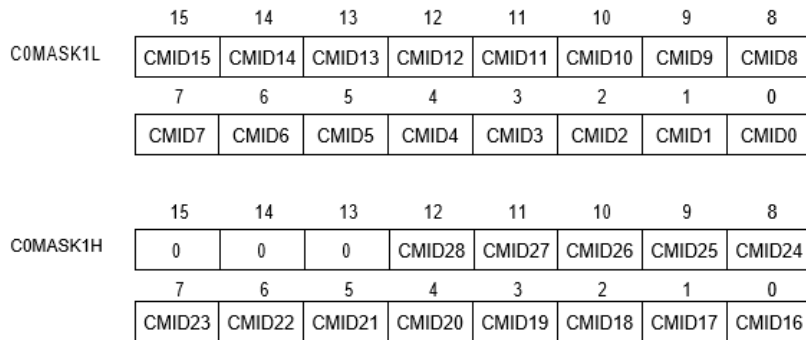
Figure 21-30. Format of the CAN module mask register (C0MASKaL, C0MASKaH) (a = 1, 2, 3, or 4) (1/2) - CAN Module Masking 1 register (C0MASK1L, C0MASK1H)
