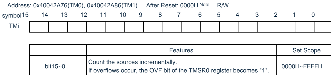
Figure 10-31 Timer M Counter i(TM i ) (i=0,1) Format [Reset Synchronous PWM Mode and PWM3 Mode]
