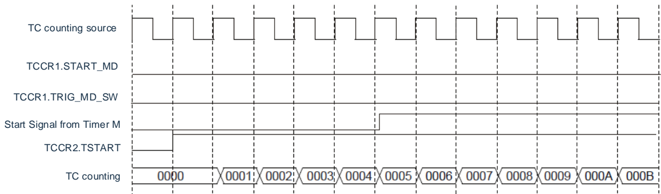
Figure 9-14 Example of Timer M triggering Timer C count reset
