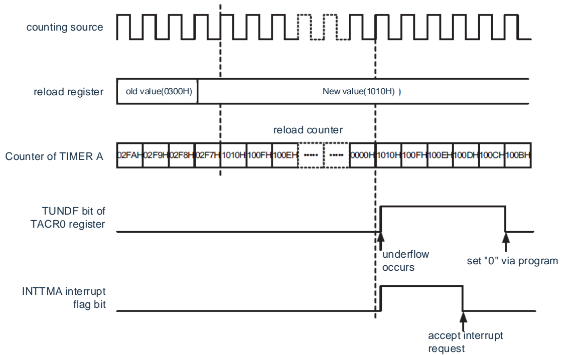
Figure 7-1 0 Running example of timer mode
