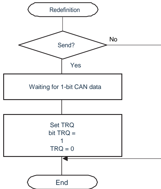
Figure 21-53. Setting Send Request (TRQ) to Send Message Cache after Redefinition
