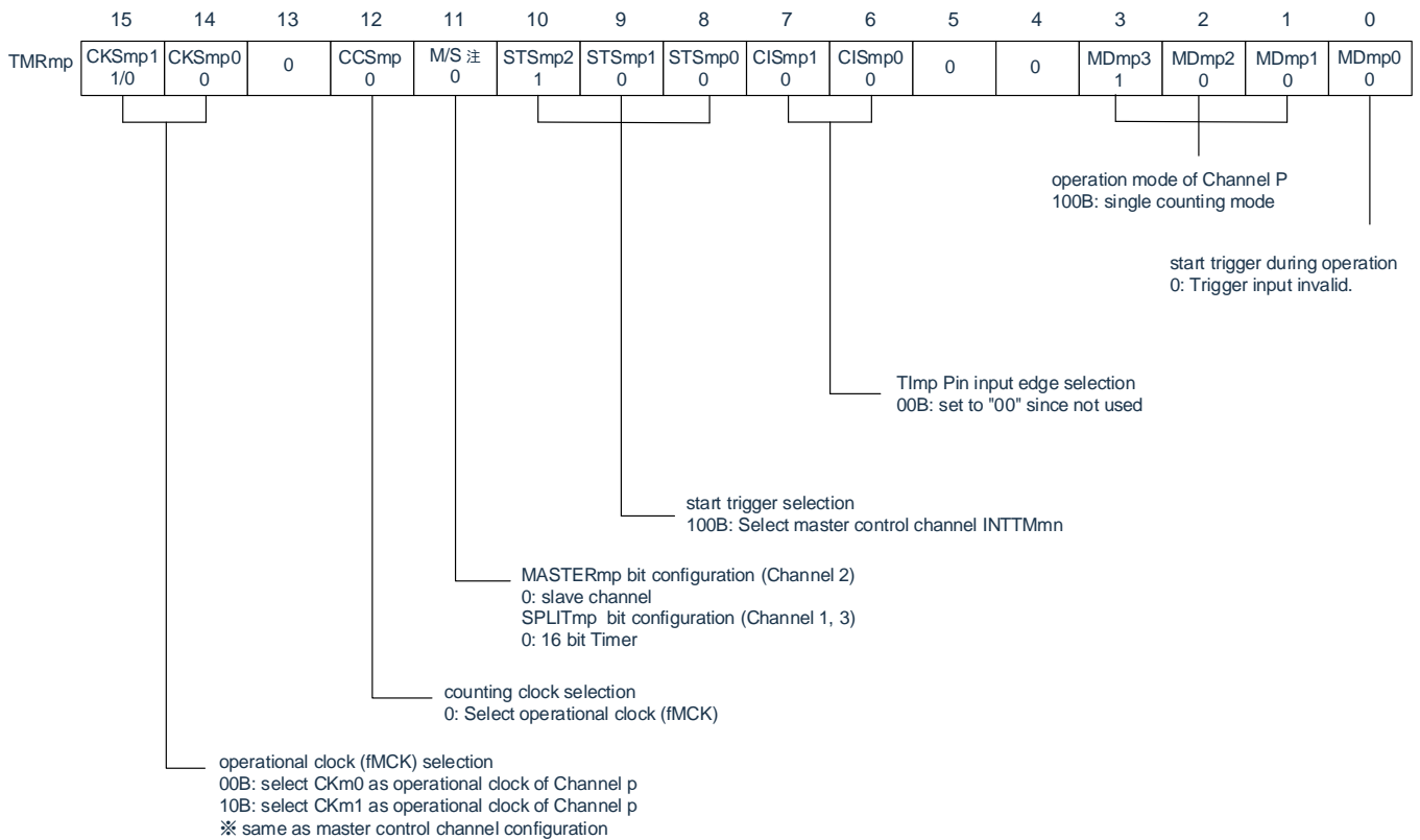
Figure 6-63 Example of Register Setting Content for Single Trigger Pulse Output Function (Slave Channel) (a) timer mode register mp (TMRmp)
