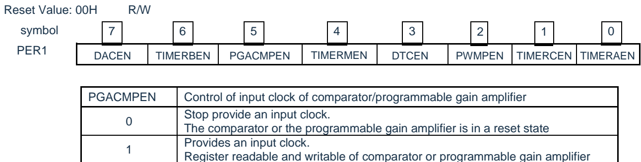
Figure 18-2 Format of Peripheral Admission Register 1 (PER1)
