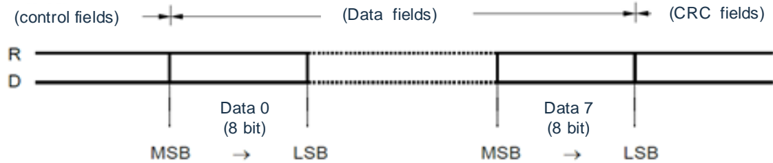
Figure 21-9. Data fields
